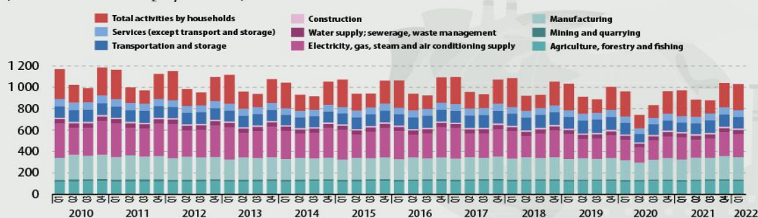
Greenhouse gas emissions by economic activity, EU, Q1 2010 - Q1 2022 (million tonnes of CO 2 equivalents)
